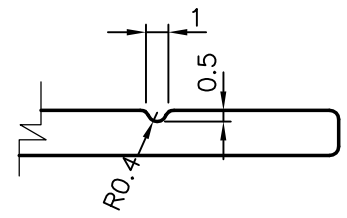
VEE GROOVE DETAIL
