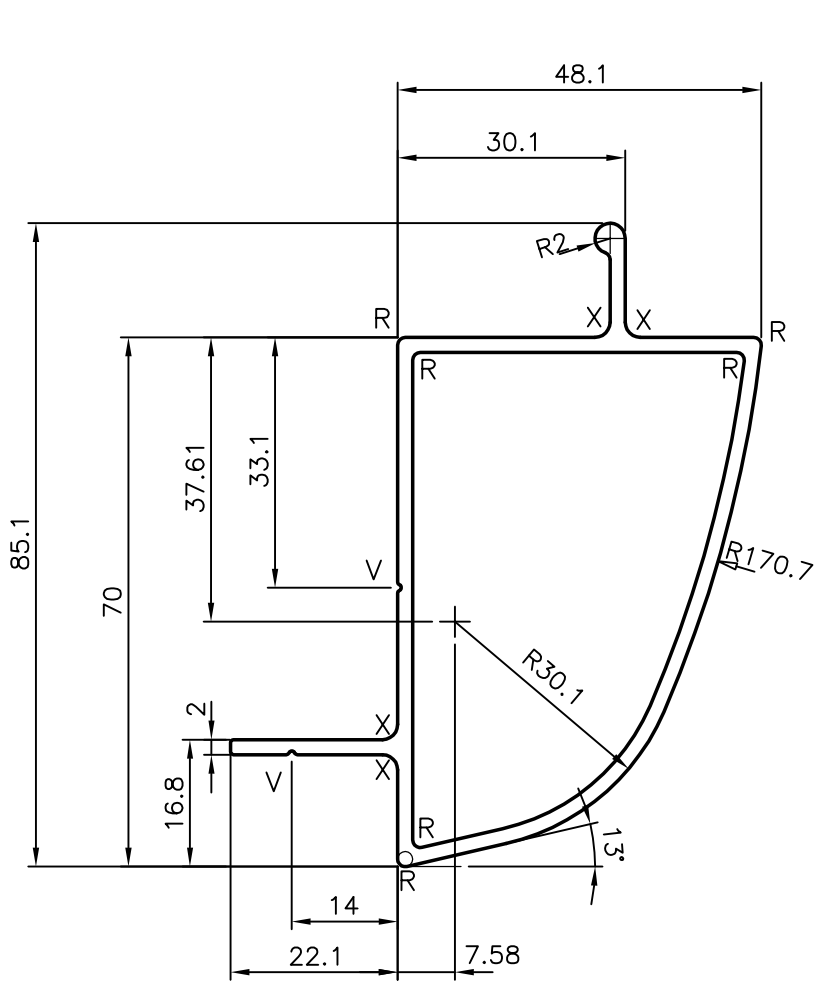
VEE GROOVE DETAIL
