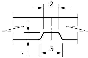
DETAIL OF "A" SCALE 4:1
