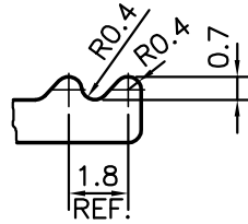
DETAIL OF "A" SCALE 4:1
