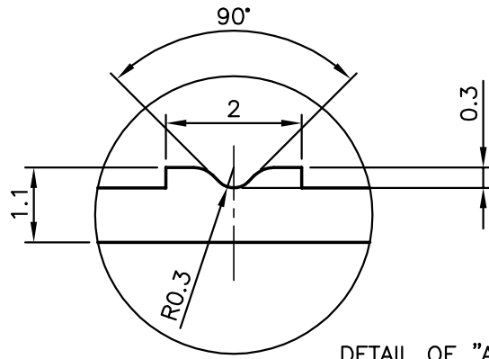
DETAIL OF "A" SCALE 10:1
