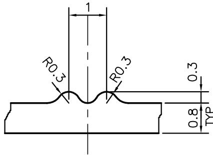
DETAIL OF "A" SCALE 10:1
