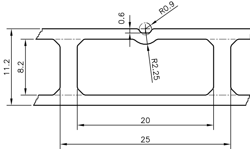
DETAIL OF "A" SCALE 3:1
