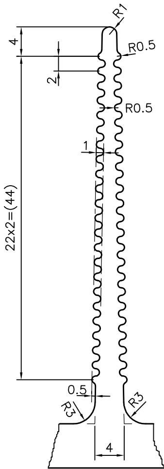
DETAIL OF "A" SCALE 2:1
