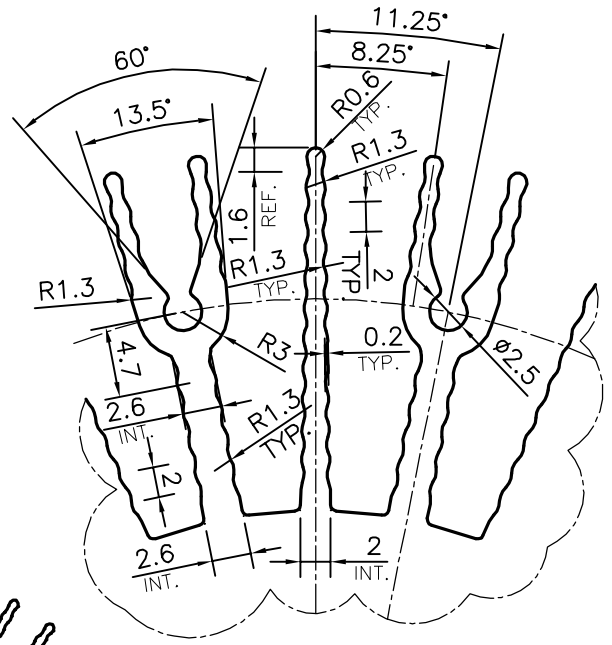
DETAIL OF "A" SCALE 2:1
