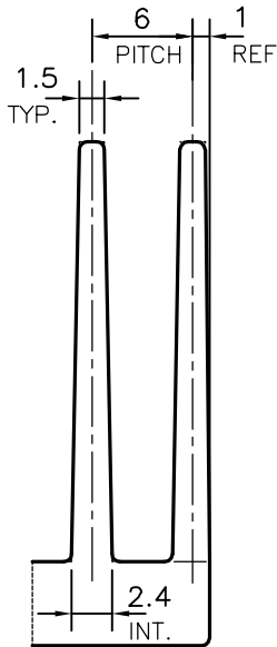
DETAIL OF "A" SCALE 2:1
