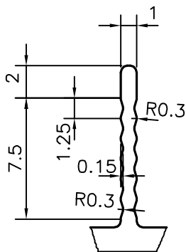
DETAIL OF "A" SCALE 3:1
