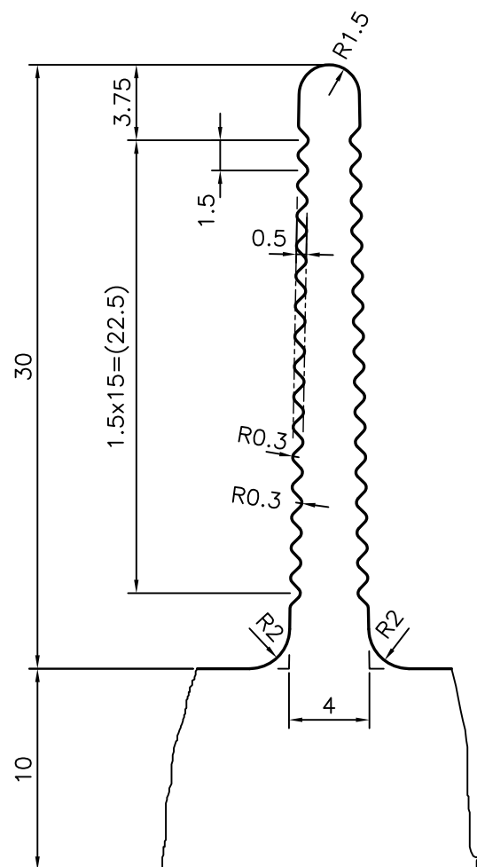
DETAIL OF "A" SCALE 3:1
