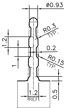
DETAIL OF "A" SCALE 5:1
