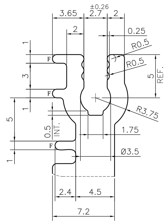
DETAIL A SCALE 4:1
