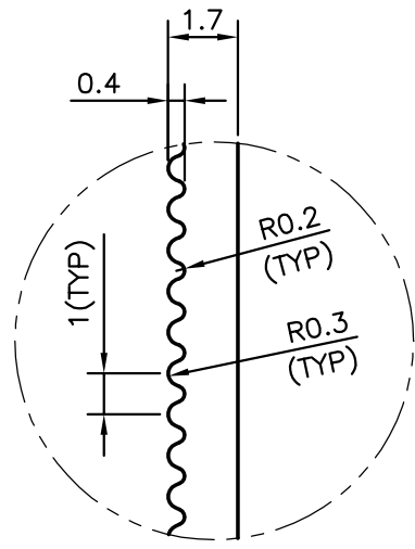
DETAIL OF "A" SCALE 5:1
