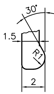
DETAIL OF "A" SCALE 5:1
