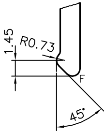
DETAILS OF "A" SCALE 3:1
