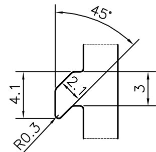
DETAIL OF "A" SCALE 3:1
