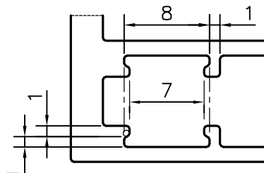
DETAIL OF "A" SCALE 2:1
