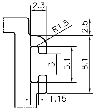
DETAIL OF "B" SCALE 3:1
