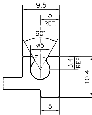
DETAIL OF "B" SCALE 2:1
