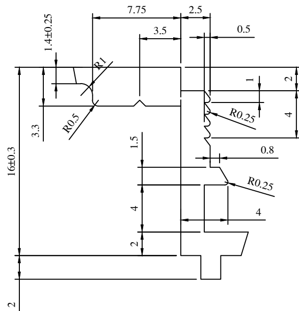
DETAIL AT-A
