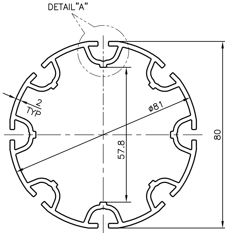
MATCHING SECTION SCALE 1:1
