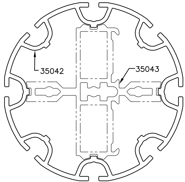
MATCHING SECTION SCALE 1:1
