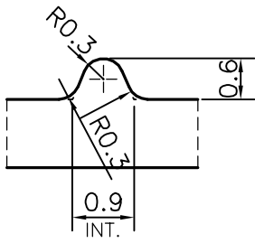
DETAIL OF "A" SCALE :- 10:1
