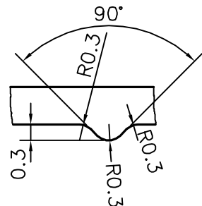
DETAIL OF PIP SCALE :- 10:1
