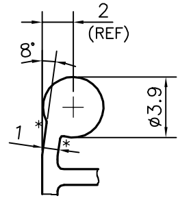
DETAILS OF "A" SCALE 3:1
