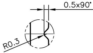
DETAIL OF "B" SCALE 4:1
