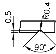
DETAIL OF 'V' GROOVE
