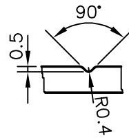
DETAIL OF 'V' GROOVE
