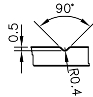
DETAIL OF V GROOVE
