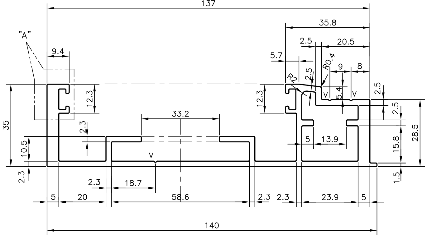
DETAIL OF "A" SCALE 2:1
