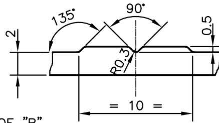
DETAIL OF "B" SCALE 3:1
