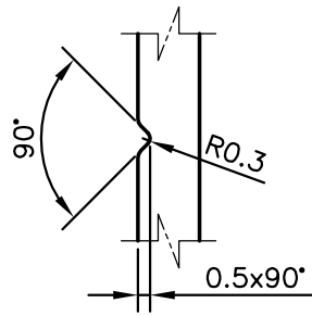
DETAIL OF 'B' SCALE 3:1
