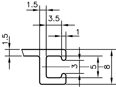
DETAIL "B" (2:1)
