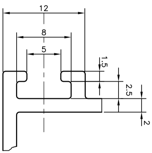
DETAIL "B" (3:1)
