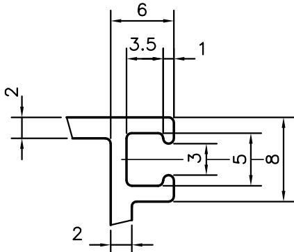
DETAIL "B" (2:1)
