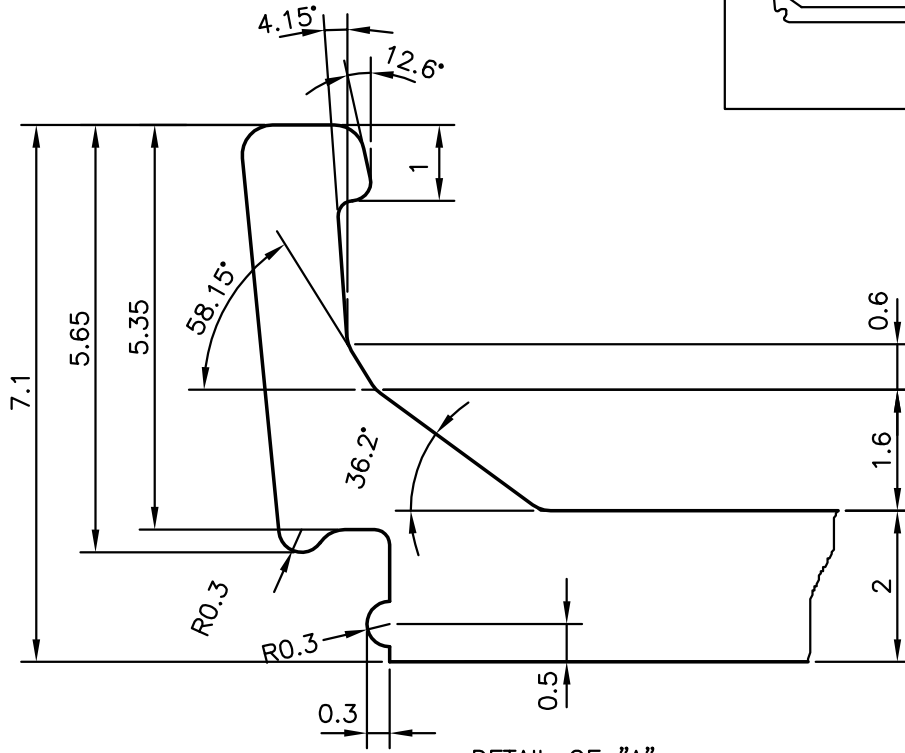
DETAIL OF "A" SCALE 10:1
