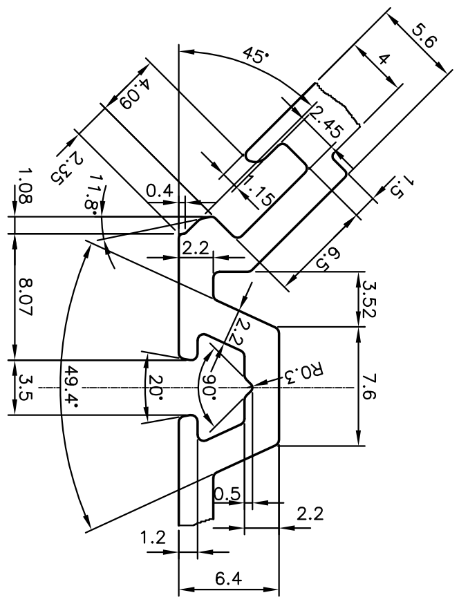
DETAIL OF "B" SCALE 3:1
