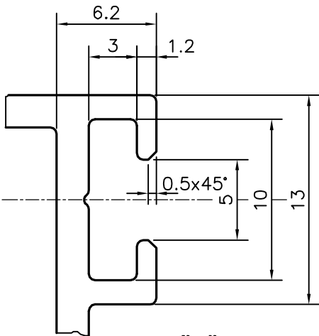
DETAIL "B" SCALE 3:1
