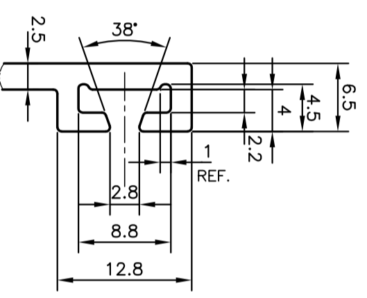
DETAIL OF "B" SCALE 2:1
