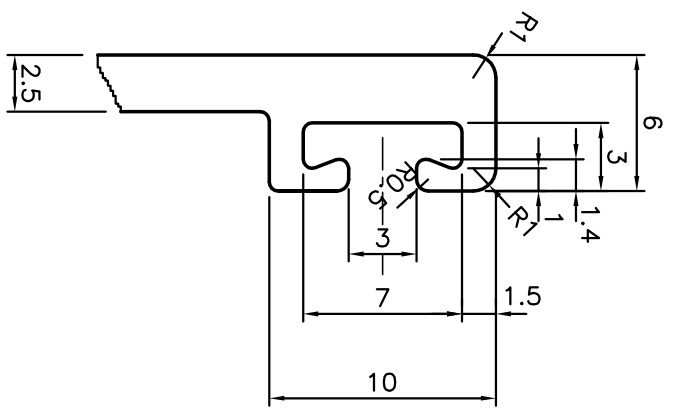
DETAIL OF "C" SCALE 3:1
