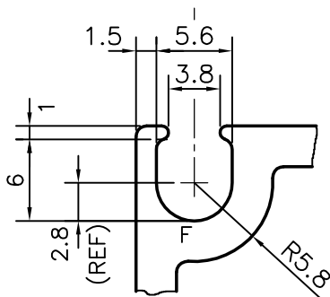
DETAILS OF "B" SCALE 2:1
