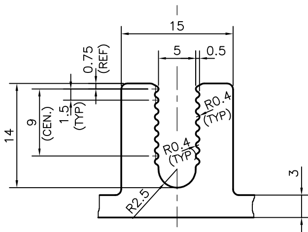
DETAILS OF "A" SCALE 2:1
