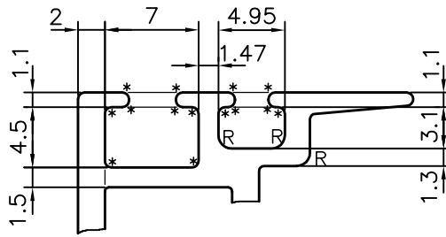
DETAIL OF "A" SCALE 2:1
