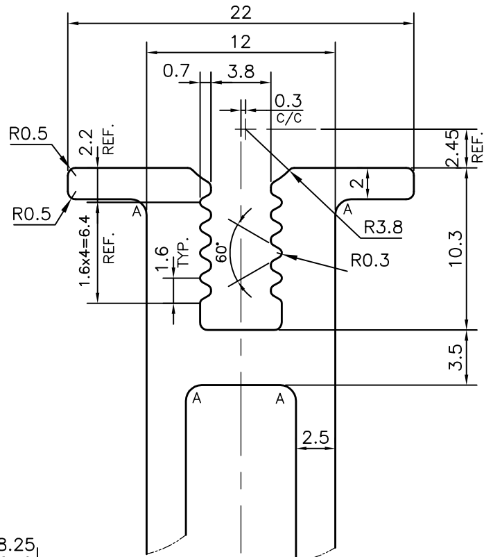
DETAIL OF "A" SCALE 3:1
