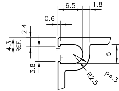
DETAIL 'A' (2:1)
