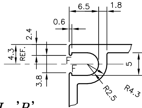
DETAIL 'A' (2:1)
