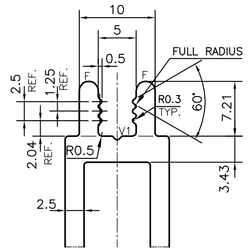
DETAIL OF "B" SCALE- 2:1
