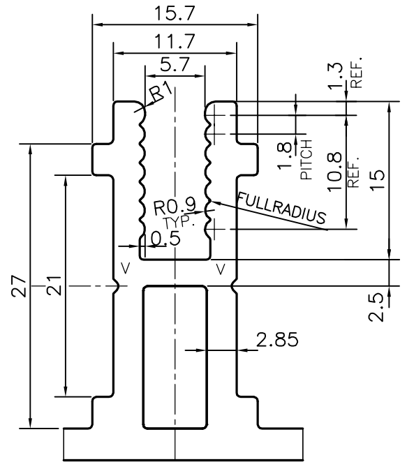
DETAIL OF 'A' SCALE :- 2:1
