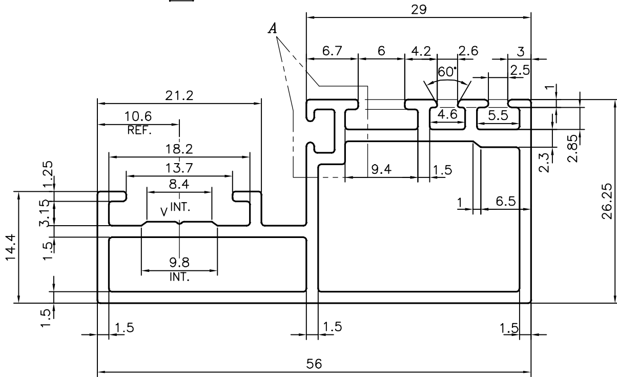
DETAIL OF "A" SCALE 4:1
