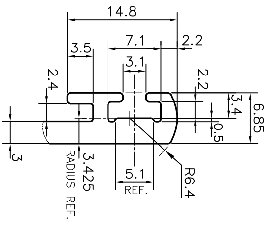
DETAIL OF "C" SCALE 2:1
