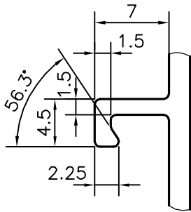
DETAIL OF "A" SCALE :- 2:1
