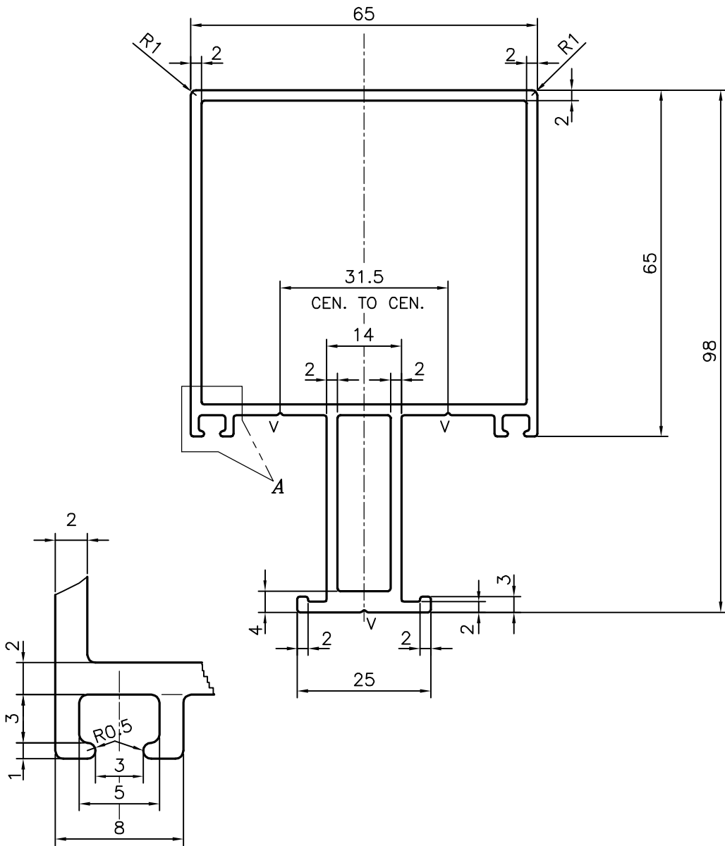
DETAIL OF "A" SCALE 3:1
