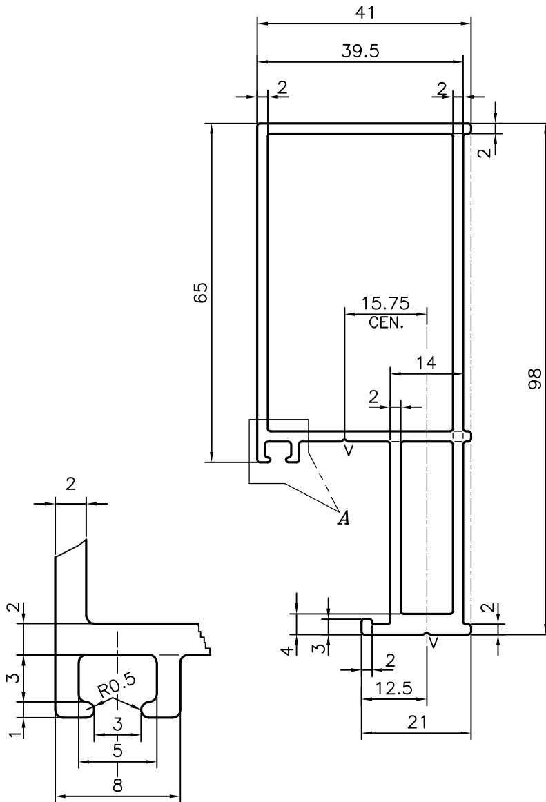
DETAIL OF "A" SCALE 3:1
